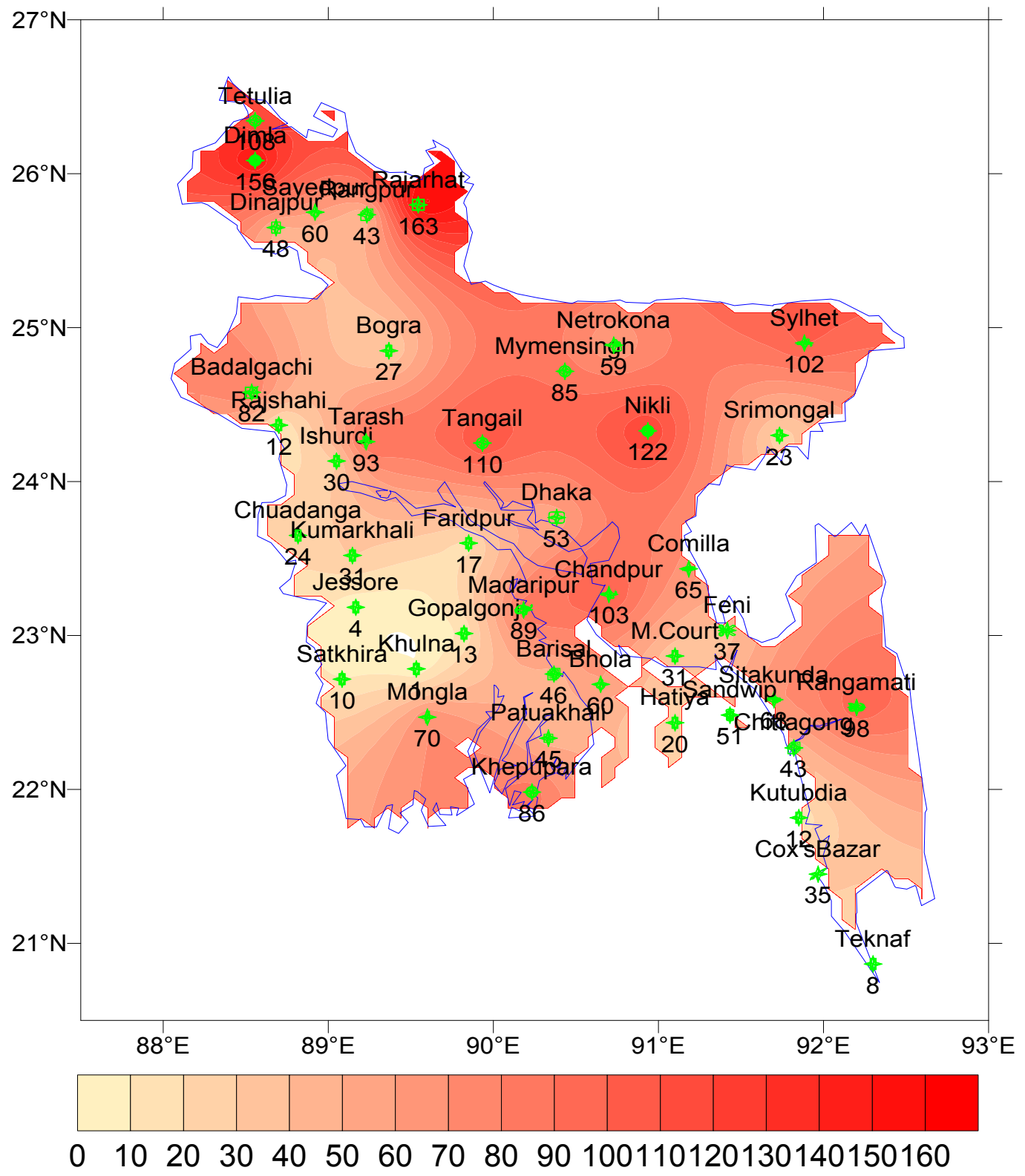
Spatial distribution of Rainfall (mm), Period (15-06-2019 to 21-06-2019)
